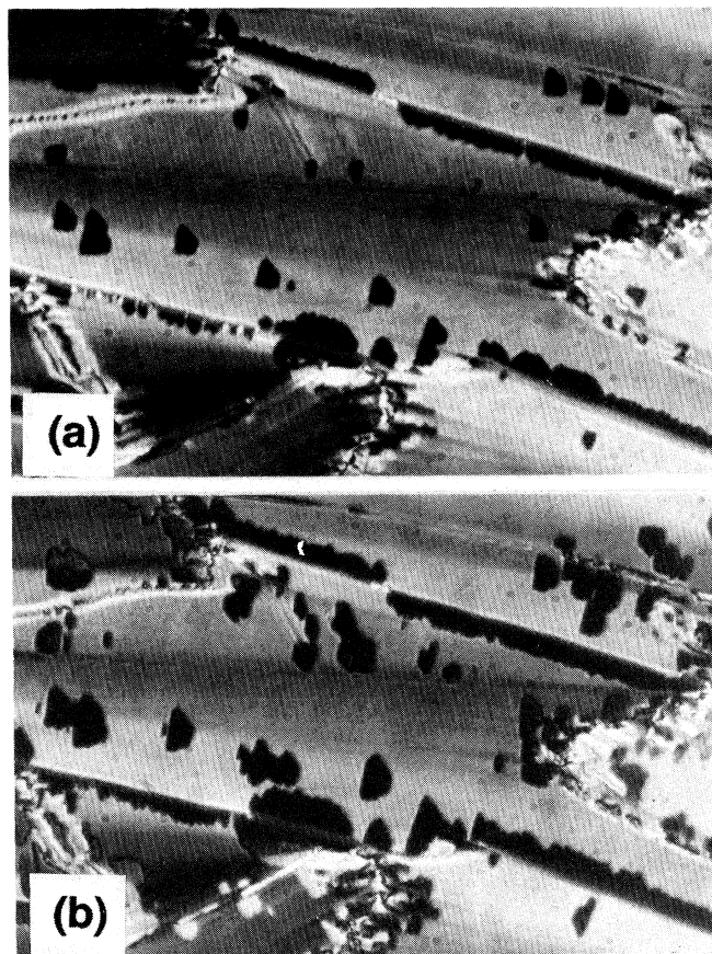
FIG. 9. Photomicrographs of the reversing domains when T = 25^\circ\text{C} . The pictures were taken when the (a) 5 V voltage is applied for 5.582 ms and (b) 8 V applied for 4.243 ms. Notice that the asymmetry of the domains is becoming less pronounced in (b).
